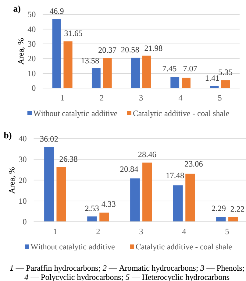
Figure 1. Component composition of the 100–200 °C light fraction (a) and 200–300 °C middle fraction (b) of hydrogenate (420 °C, 60 min, 4 MPa, ratio 0.13)
