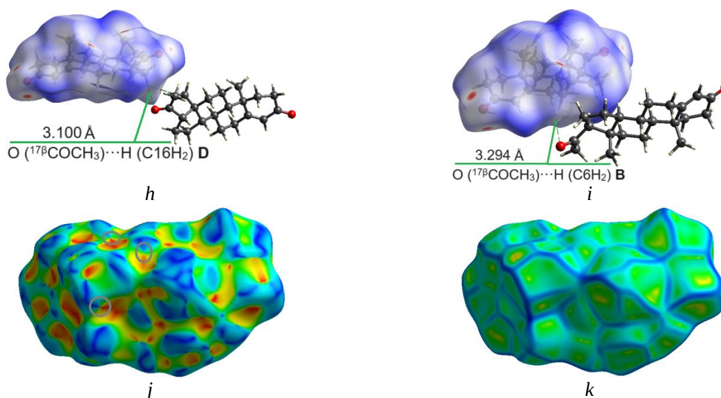
Figure 2. Progesterone crystal cell (a) and Hirschfeld surfaces mapped with d_{\text{norm}} (b–i), shape index (j) and curvedness (k). \text{CH} \cdots \text{O} intermolecular interactions are shown by green dashed lines with indicated experimental values of intermolecular contact lengths
