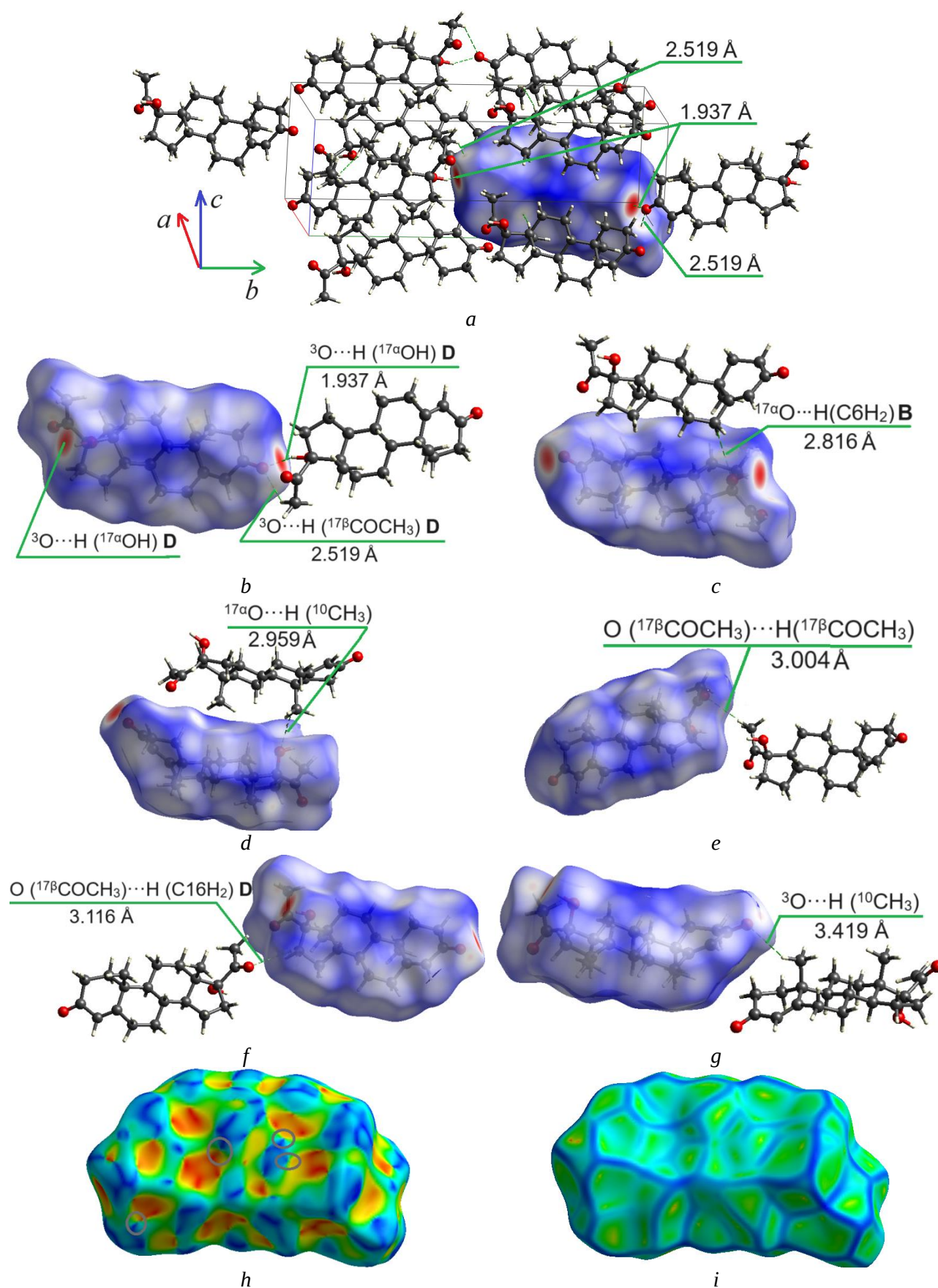
Figure 4. Crystal cell and Hirshfeld surface ( d_{\text{norm}} ) for 17 \alpha -hydroxyprogesterone (a), selected dimer configurations with indicated intermolecular distances (b-g), shape index (h), and curvedness (i)
