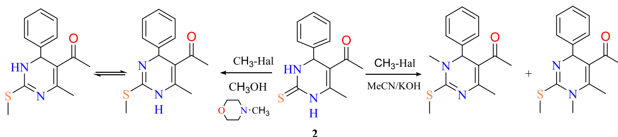
Scheme 2. Alkylation reaction of 2 in methanol with N-methylmorpholine
